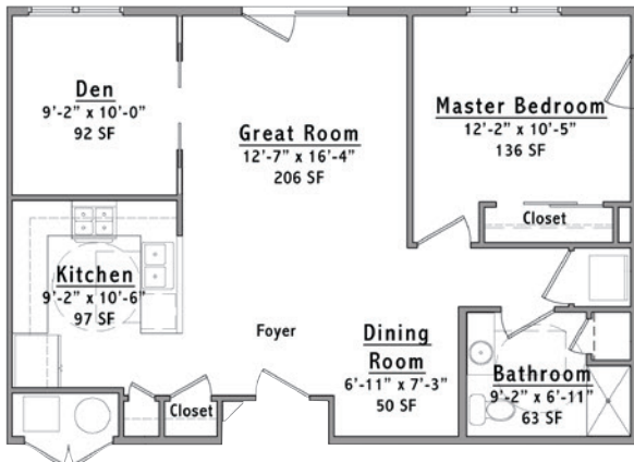
Floor Plan A (806 sq. ft.)
